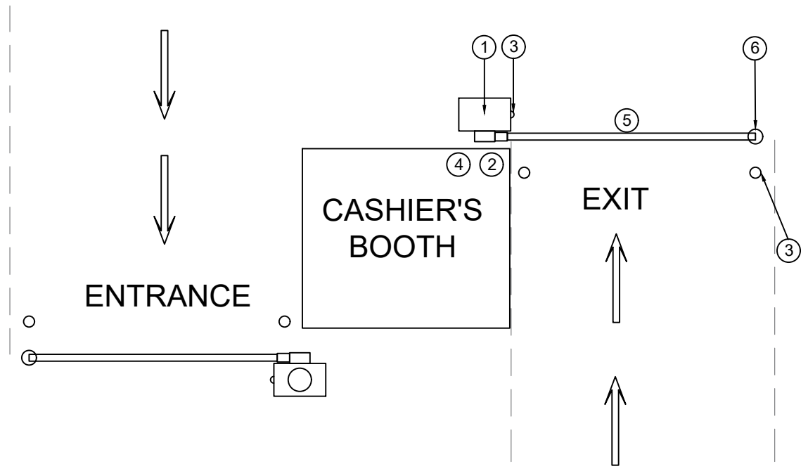
B INSTALLATION PLAN SCALE: 2/2 NTS
