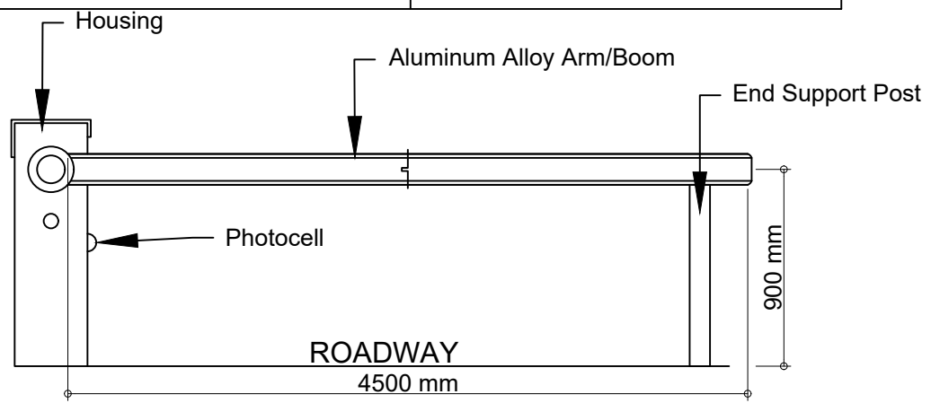
A BOOM BARRIER GATE DETAILS SCALE: 2/2 NTS
