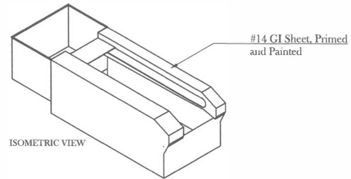
Body Cover Details Scale..... 1:30
