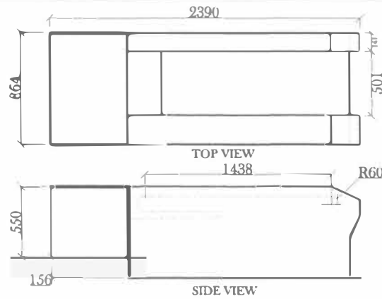
Body Cover Details Scale..... 1:30
