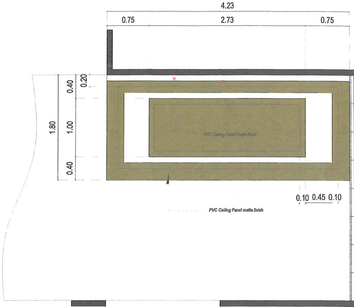
REFLECTED CEILING PLAN SCALE 1:40 MTS.
