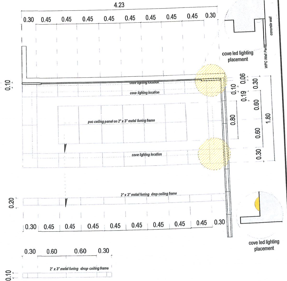
CEILING FRAME PLAN SCALE 1:40 MTS.
