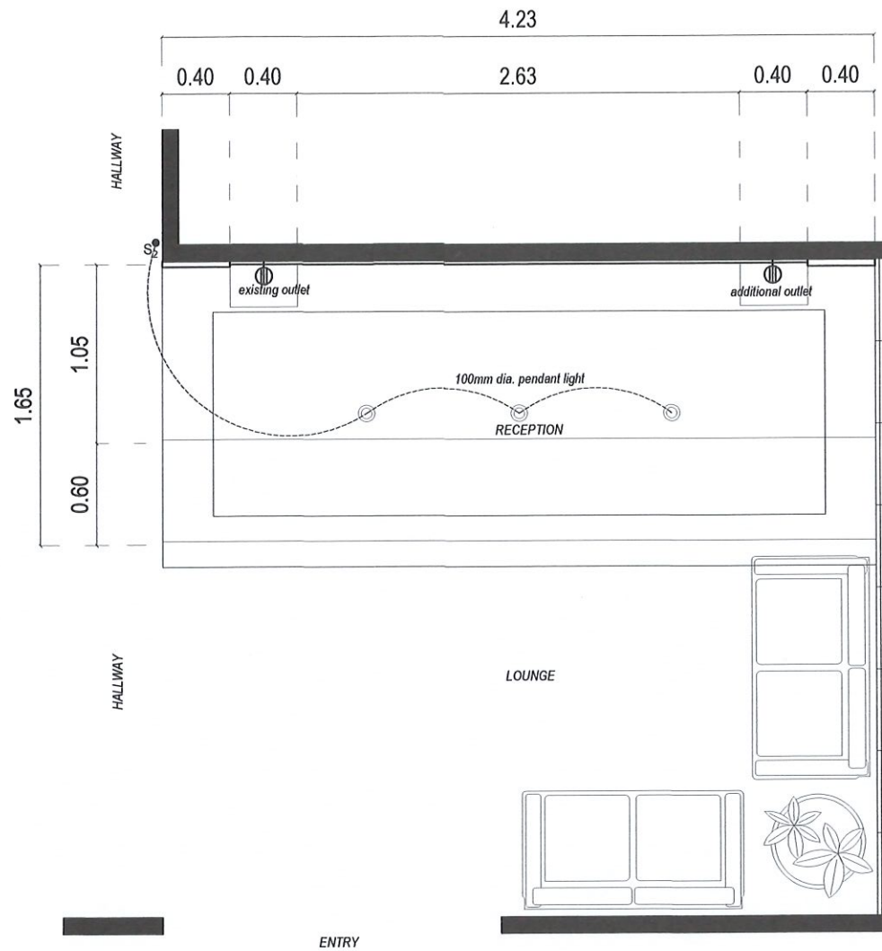
LIGHTING and POWER LAYOUT SCALE 1 : 4 0 M T S .
