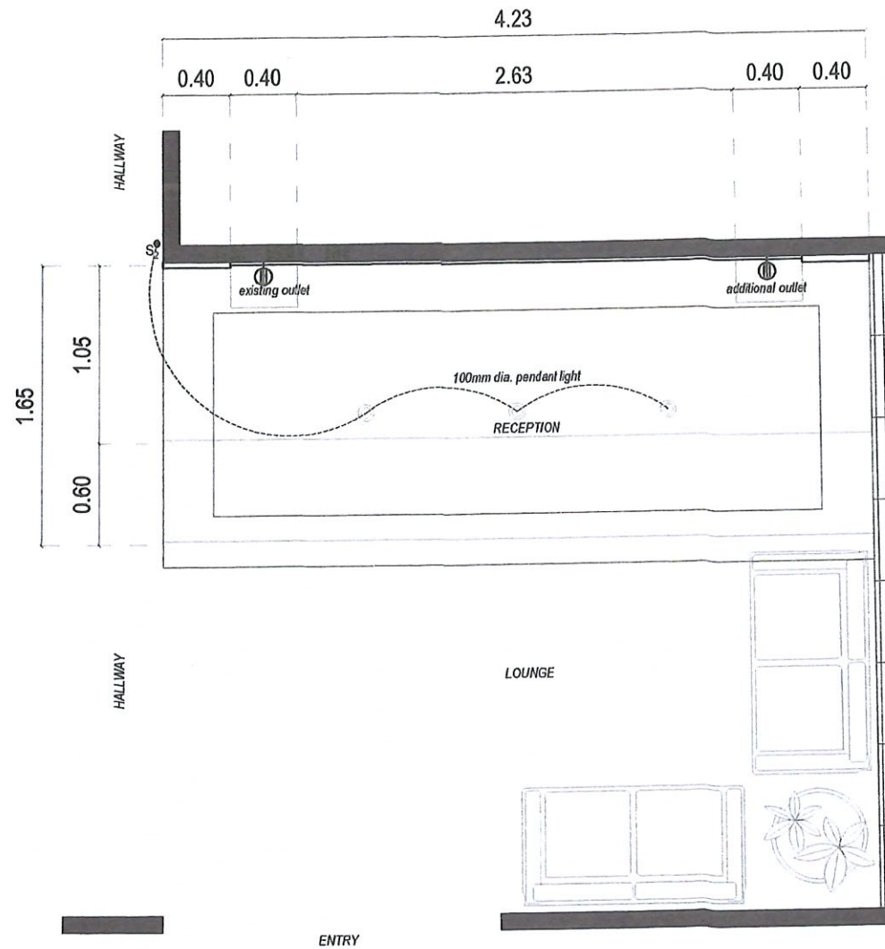
E 11 LIGHTING and POWER LAYOUT SCALE 1 : 4 0 M T S .
