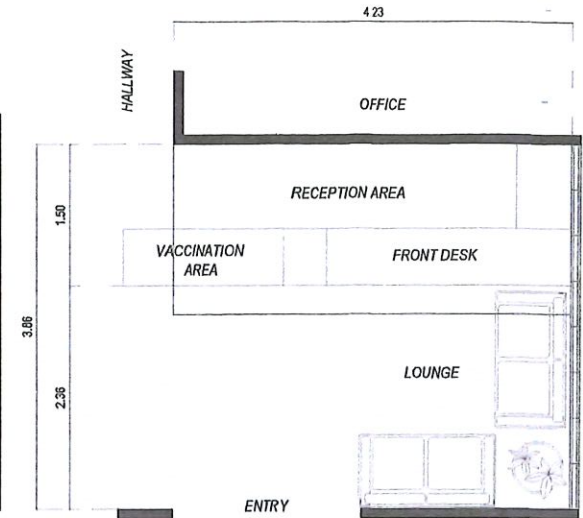
EXISTING FLOOR PLAN SCALE 1: 80 meters
